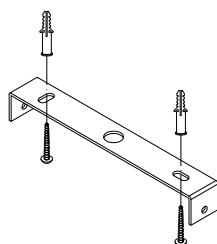
3. Apply plastic anchors, With screws
