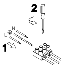
5. Connect wires
