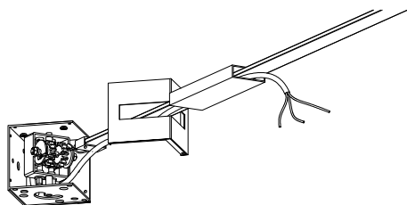
1. Pass the power cord through the decorative parts
