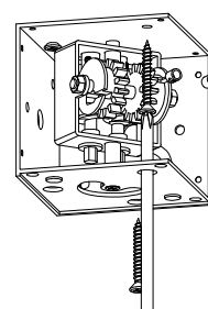
6. Install support seat
