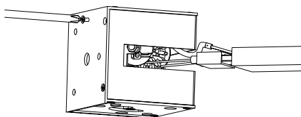
11. Install the decorative cover
