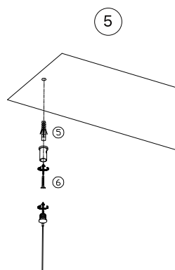
Apply plastic anchors & fix In place the hanging element
