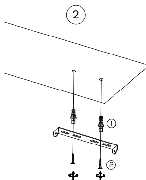
Drill holes & apply plastic anchors With screws
