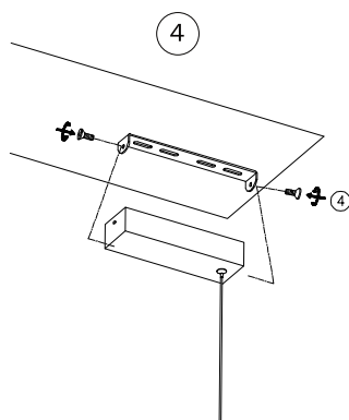
Apply the side screws
