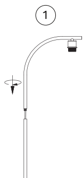
Fasten the crooked metal tube with the straight metal tube
