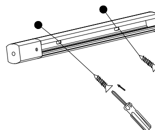
4. Apply screws
