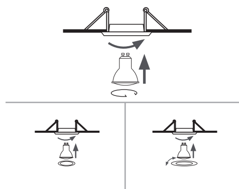
6. Apply the bulb by rotating & fix the cup
