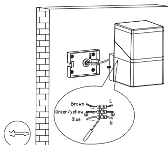
7. Connect the wires.
