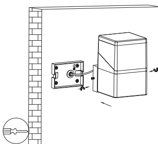
8. Connect the lamp body to the Lamp base.
