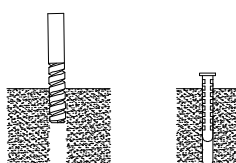
5&6. Drill on the marked areas & Apply plastic anchors.
