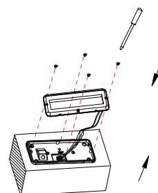
10. Install the PC cover.
