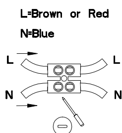
9. Connect the wires.
