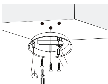
5. Apply screws
