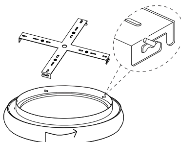
8. Apply the product by rotating
