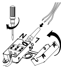
7. Connect the wires
