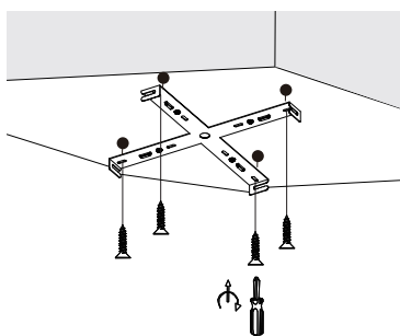
5. Apply screws
