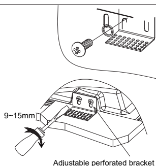
5. Apply screws into brackets
